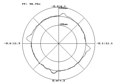
Circle after feed-forward adjustment
