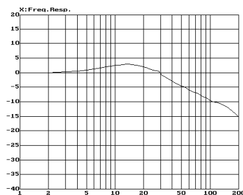
Frequency characteristic measurement results
