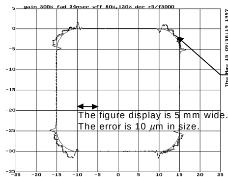
Fig. 3.4.3 (o) Arc radius based feedrate clamping
