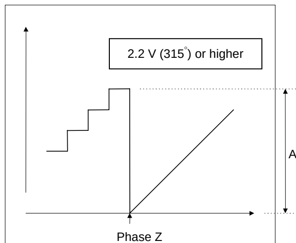
Fig. 4.14.1 (b) If the offset is set with a negative number
