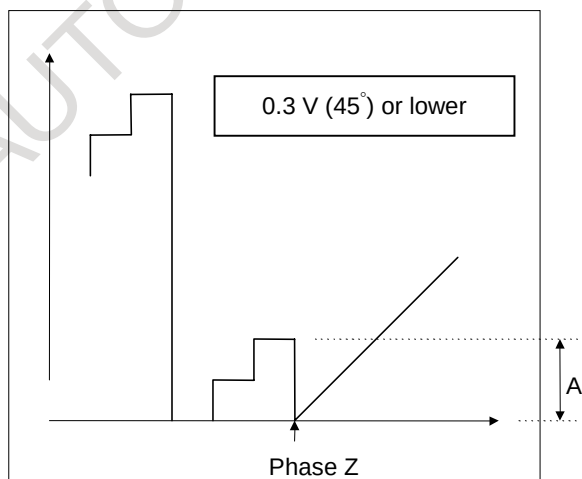
Fig. 4.14.1 (a) If the offset is set with a positive number
