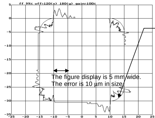
Fig. 3.4.3 (k) Velocity feed-forward adjustment
