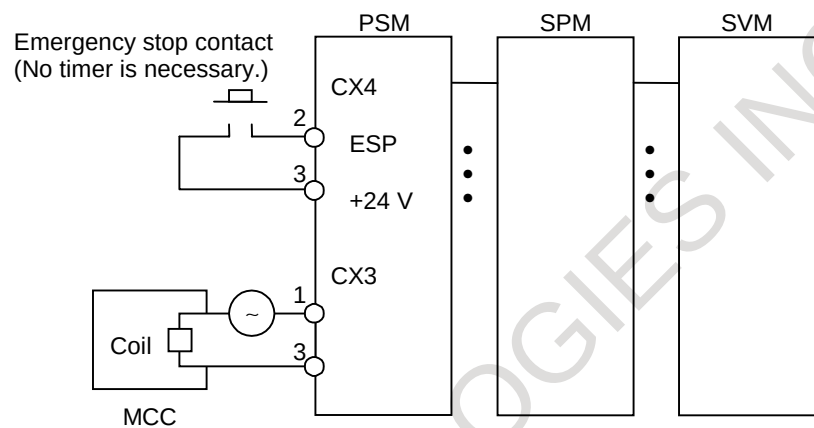
Fig. 4.11.1 (b) \alpha series amplifier
