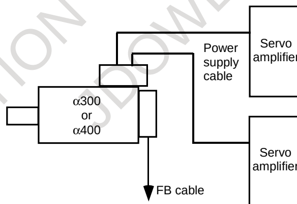
Fig. 4.17 (d) Example of exercising tandem control (winding tandem)
