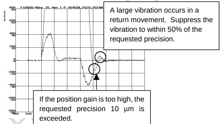
Fig. 3.4.4 (f) Excessively high position gain
