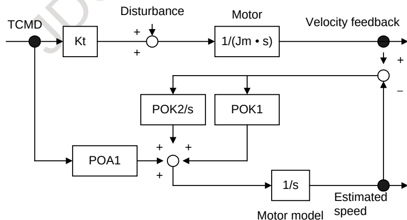
Fig. 4.5.2 (b) Block diagram of the observer
