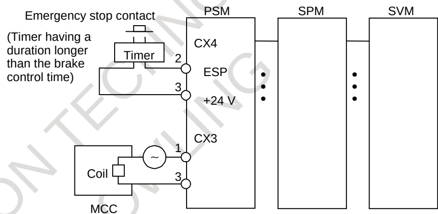
Fig. 4.10 (b) \alpha series amplifier
