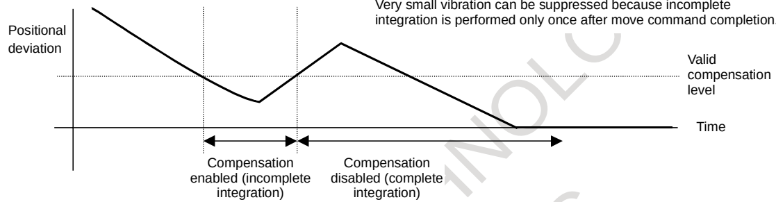
Fig. 4.7 (i) Overshoot compensation type 2
