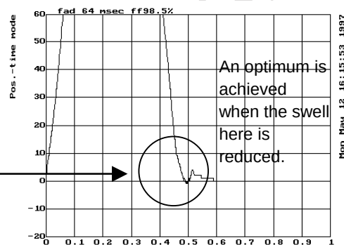
Fig. 3.4.5 (g) After velocity feed-forward adjustment
