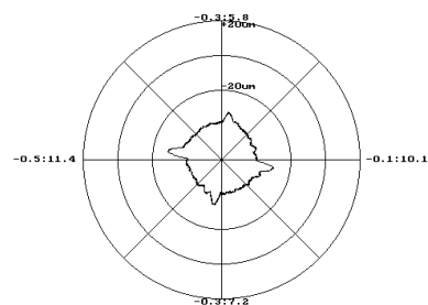
Circle before feed-forward adjustment
