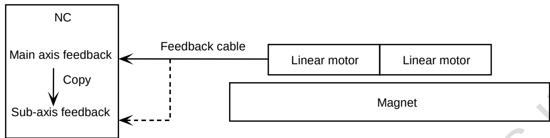
Fig. 4.17.5 Motor feedback sharing function
