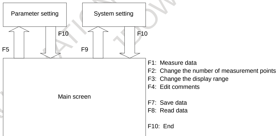
Fig. 4.19 (e) Servo adjustment software basic configuration and key manipulation
