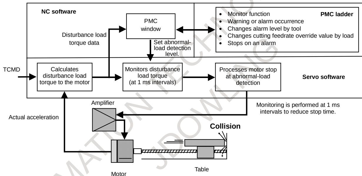
Fig. 4.12.1 Overview of abnormal-load detection
