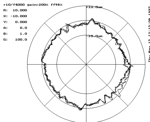
Fig. 3.4.3 (c) Effect of velocity loop gain
