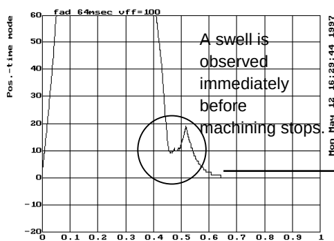
Fig. 3.4.5 (f) Before velocity feed-forward adjustment
