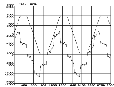
Before inertia estimation (Up: TSA, Low: Friction torque)
