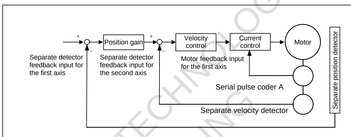
Fig. 4.16 Special system for super-precision machining
