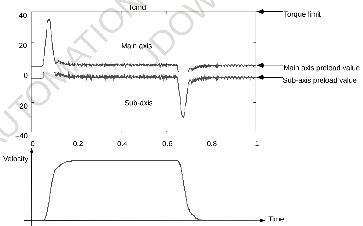
Fig. 4.17.7 (f) Tcmd at acceleration/deceleration time (when the full preload function is used)
