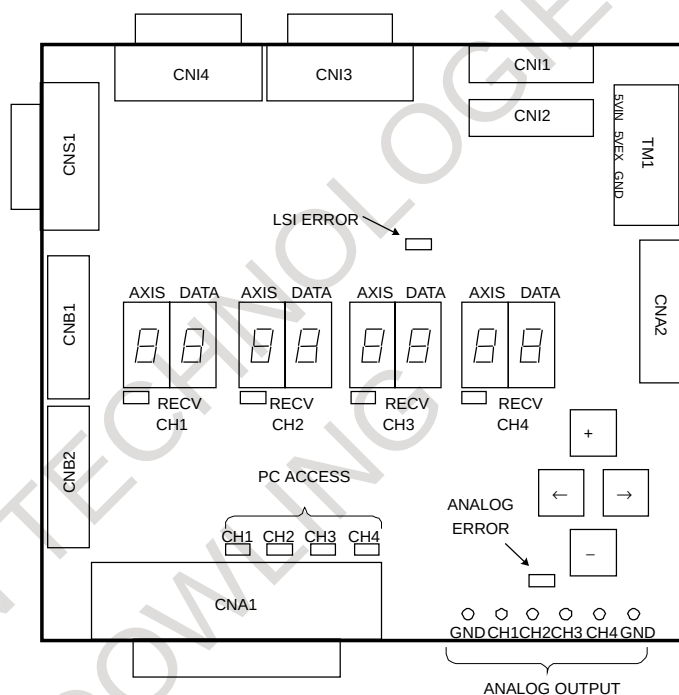
Fig. 4.19 (a) Connector layout on servo check board A (A06B-6057-H630)
