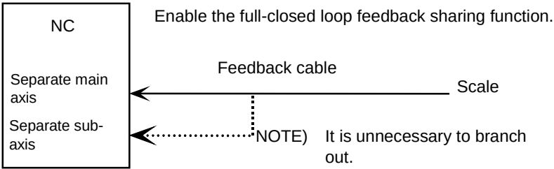
Fig. 4.17.8 (c) Example of using the full-closed loop feedback sharing function together with the position feedback switch function
