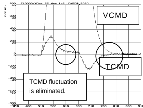
Fig. 3.4.4 (c) After velocity loop gain adjustment
