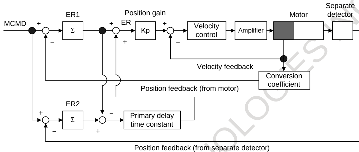
Fig. 4.5.4 Block diagram of dual position feedback control
