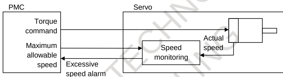
Fig. 4.15 (a) Torque control type 1
