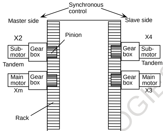
Fig. 4.17.7 (e) Synchronous tandem control
