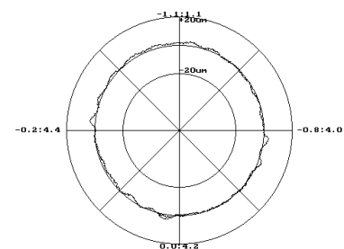
Circle after backlash acceleration adjustment
