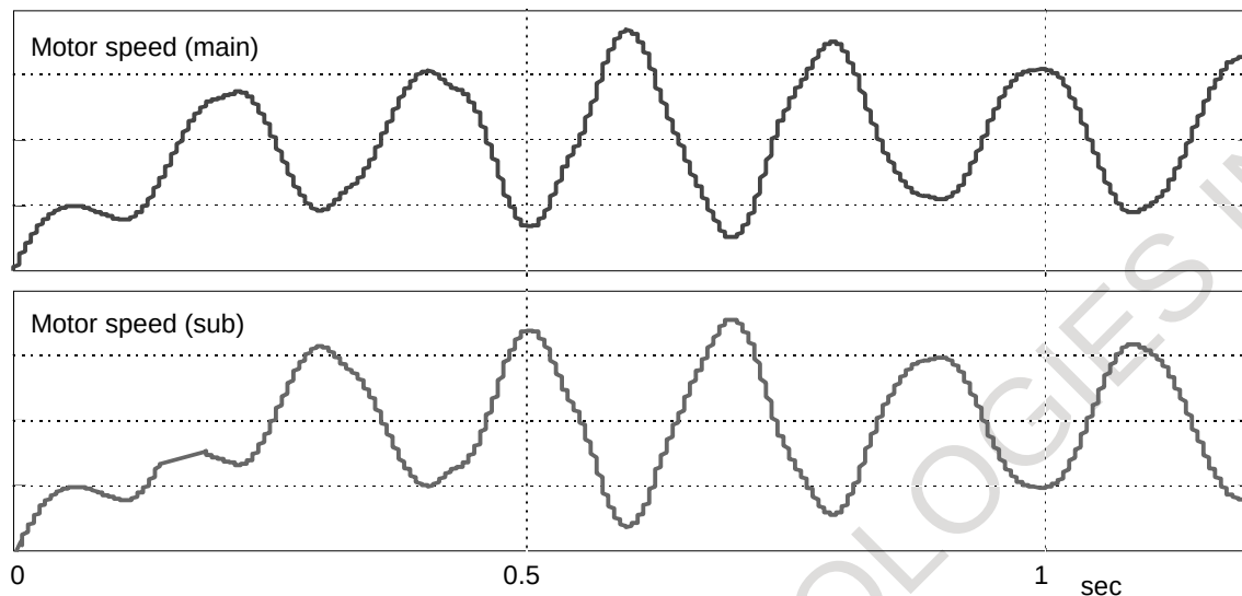
Fig. 4.17.2 (b) Motor speed vibration
