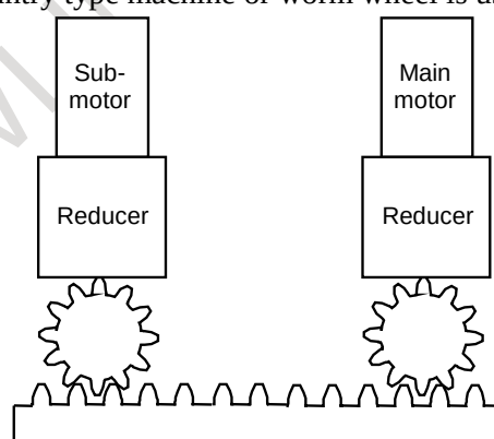
Fig. 4.17.10 (c) Example of tandem control (machine system supporting back-feed)
