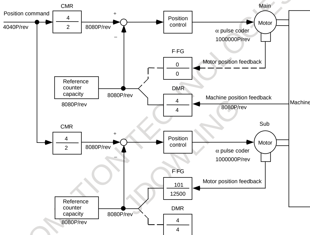
Fig. 4.17.9 (a) Example of position feedback setting
