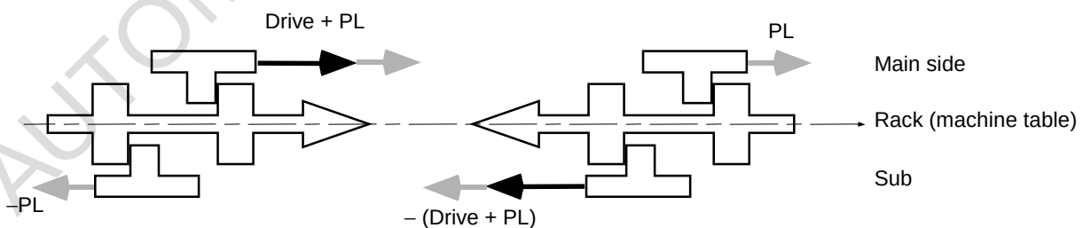
Fig. 4.17.7 (b) Relationship between full preloads and backlash (conceptual)
