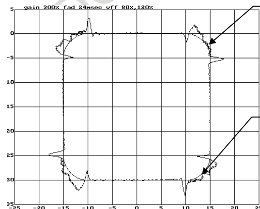
Fig. 3.4.3 (l) Velocity feed-forward adjustment
