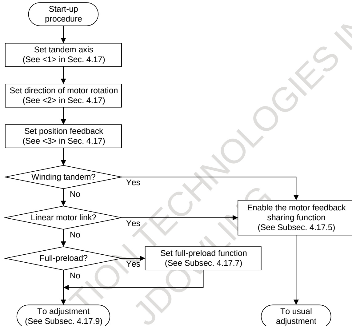
Fig. 4.17 (e) Start-up procedure flowchart
