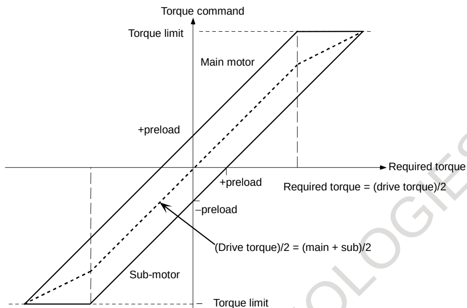
Fig. 4.17.1 (b) Relationship between required torque and torque command for each motor
