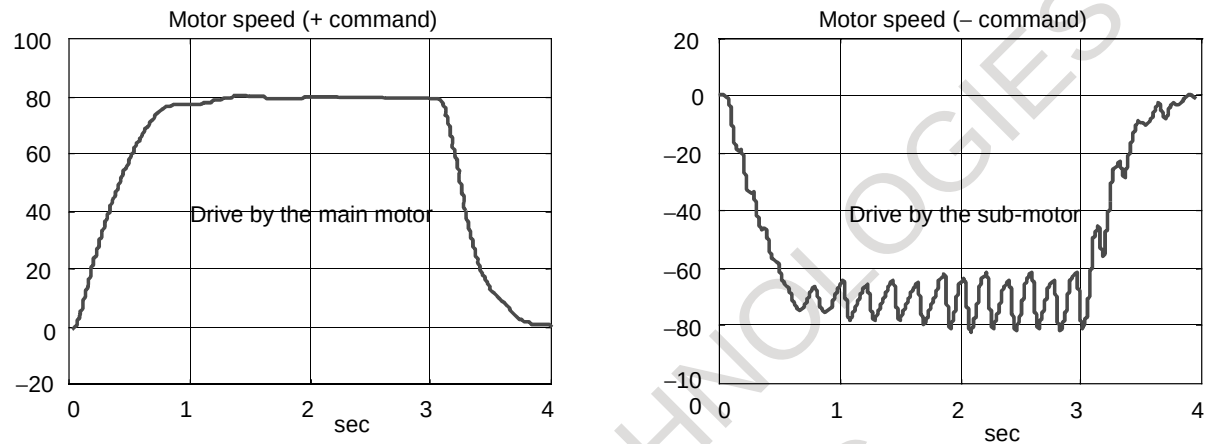
Fig. 4.17.8 (a) Motor speeds with plus-direction and minus-direction commands
