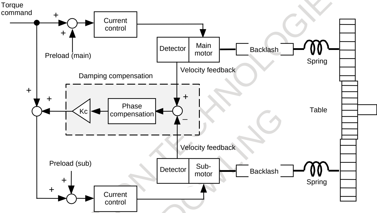
Fig. 4.17.2 (a) Damping compensation function
