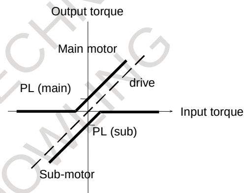
Fig. 4.17.7 (a) Full preload function
