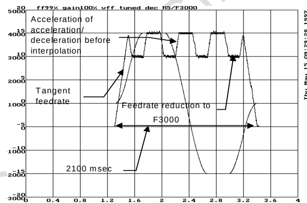
Fig. 3.4.3 (n) When the arc radius based feedrate clamp function is used
