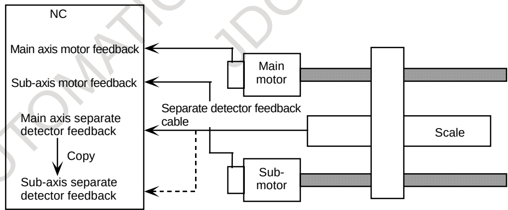
Fig. 4.17.6 Full-closed loop feedback sharing function
