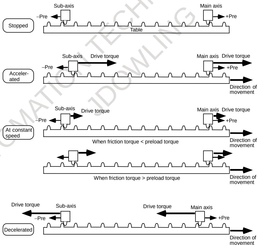
Fig. 4.17.1 (a) Changes of torque during movement
