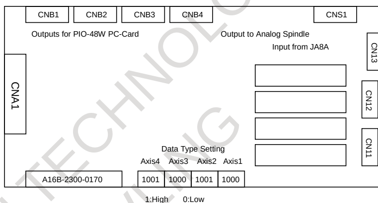
Fig. 4.19 (b) Connector layout on servo check board B (A06B-6057-H620)
