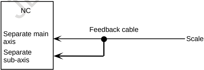
Fig. 4.17.8 (b) Cable on the scale side when the position feedback switching function is used (full-closed loop)
