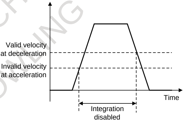
Fig. 4.8.1 (b) Integration invalid range at low-speed integration
