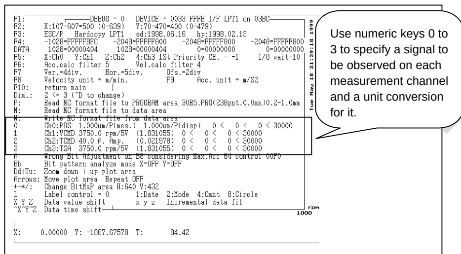
Fig. 4.19 (f) System setting screen
