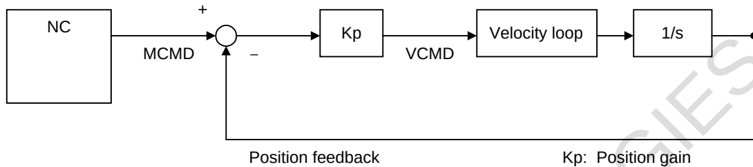
Fig. 4.7 (a) Digital servo system configuration
