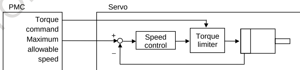
Fig. 4.15 (b) Torque control type 2
