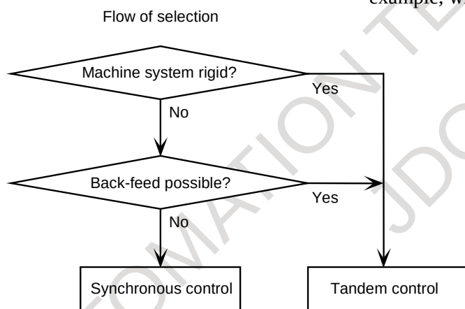
Fig. 4.17.10 (a) Flow of selection
