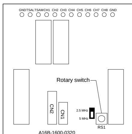
Fig. 4.19 (c) Connector layout on servo check board C (A06B-6057-H602)
