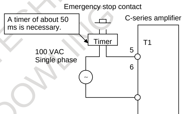
Fig. 4.11.1 (c) C-series amplifier
