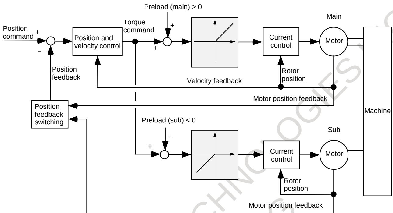
Fig. 4.17.7 (c) Servo block diagram (full preload function)
